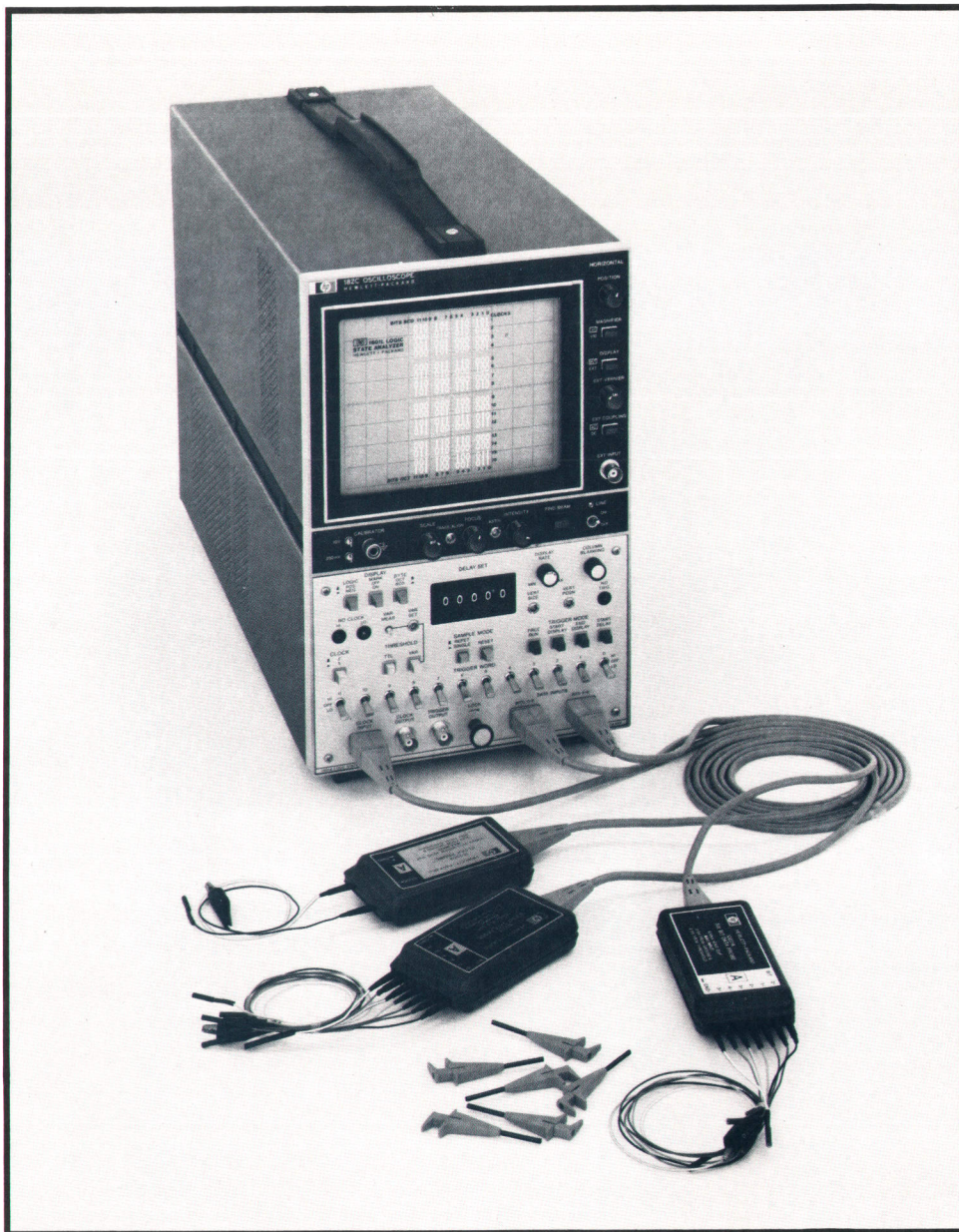
Fig. 1. Model 1601L Logic State Analyzer system displays program flow in a digital processor in an easy-to-comprehend tabular form, greatly easing the task of finding troubles in a digital system. The Model 182C Oscilloscope mainframe supplied with the system is a standard unit that can be used with other plug-ins. Conversely, the Logic State Analyzer plug-in can be used with other mainframes in the 180 family.
