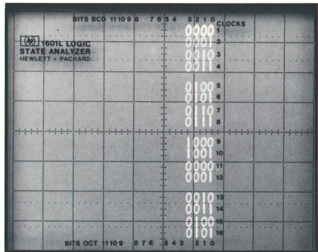
Fig. 3. State flow in a BCD counter. The trigger word at the top is brightened indicating here that the CRT displays the trigger and the 15 states that follow the trigger. The numerical scales, silk-screened on the back side of the contrast filter, assist in identifying states.
