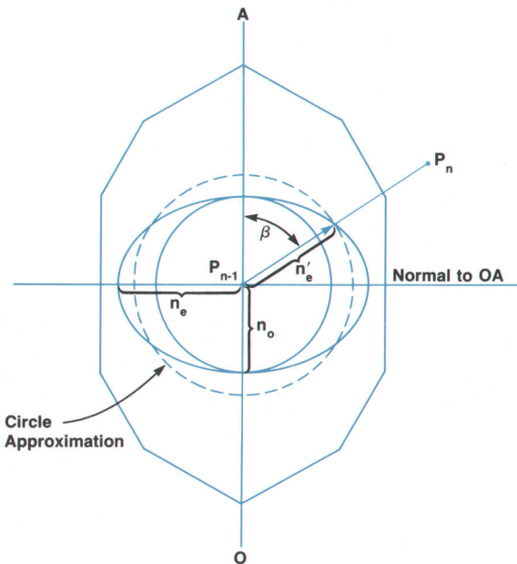
Fig. B. The extraordinary index in a uniaxial material, such as quartz, is a function of the angle between \overline{P_{n-1}P_n} and the optic axis and can be approximated using a circle method. The ellipse has rotational symmetry about the optic axis OA.
