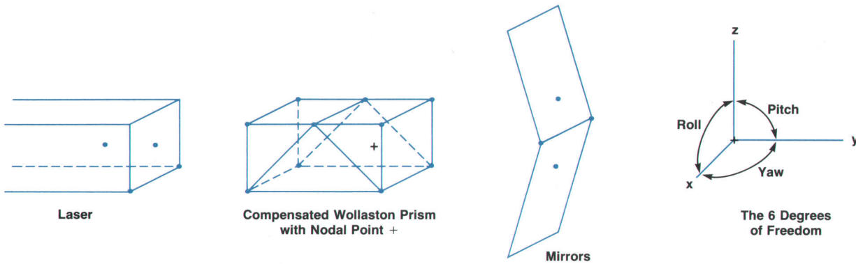
Fig. C. The short-range straightness interferometer program creates a three-dimensional model of the system, using points in space. All movement will occur about a user-defined point.
